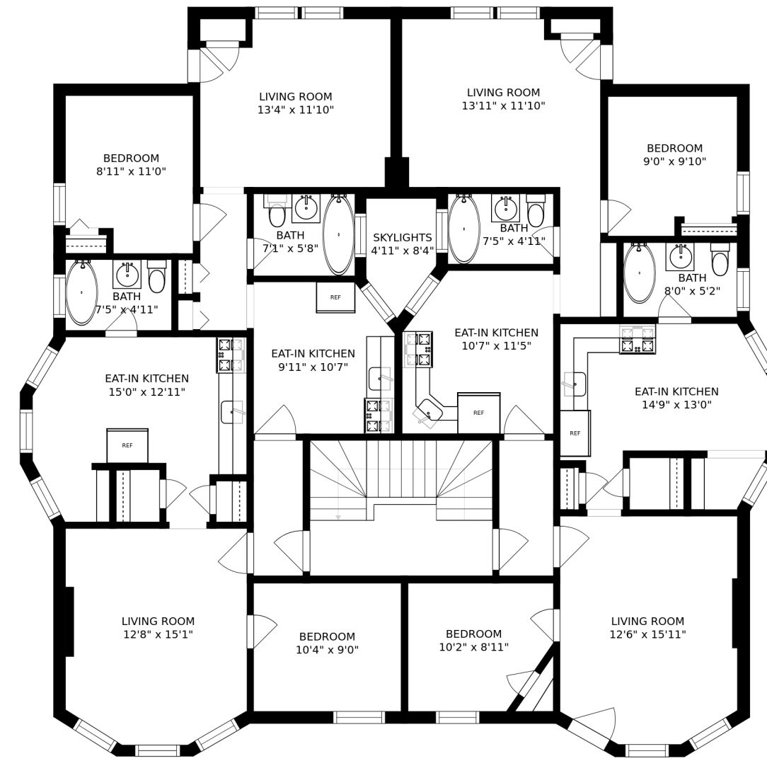
FLOOR 2
