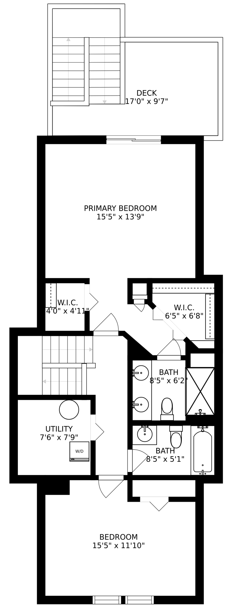
FLOOR 4
