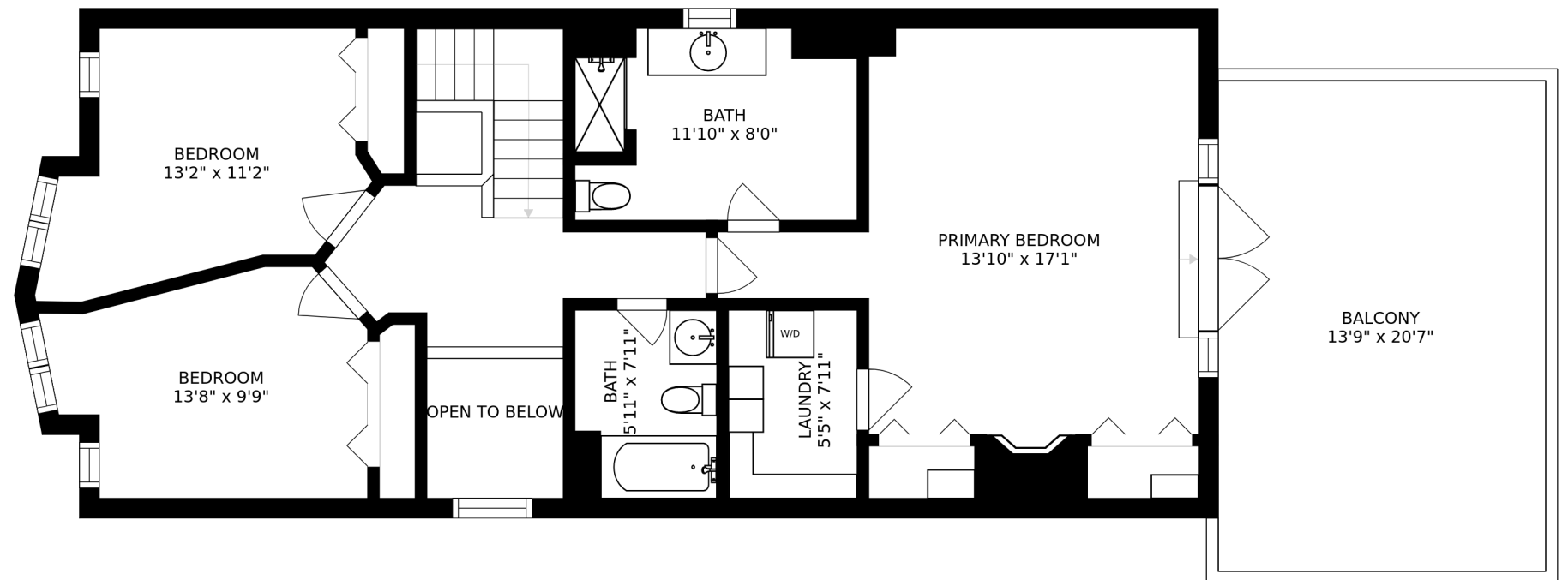
FLOOR 4
