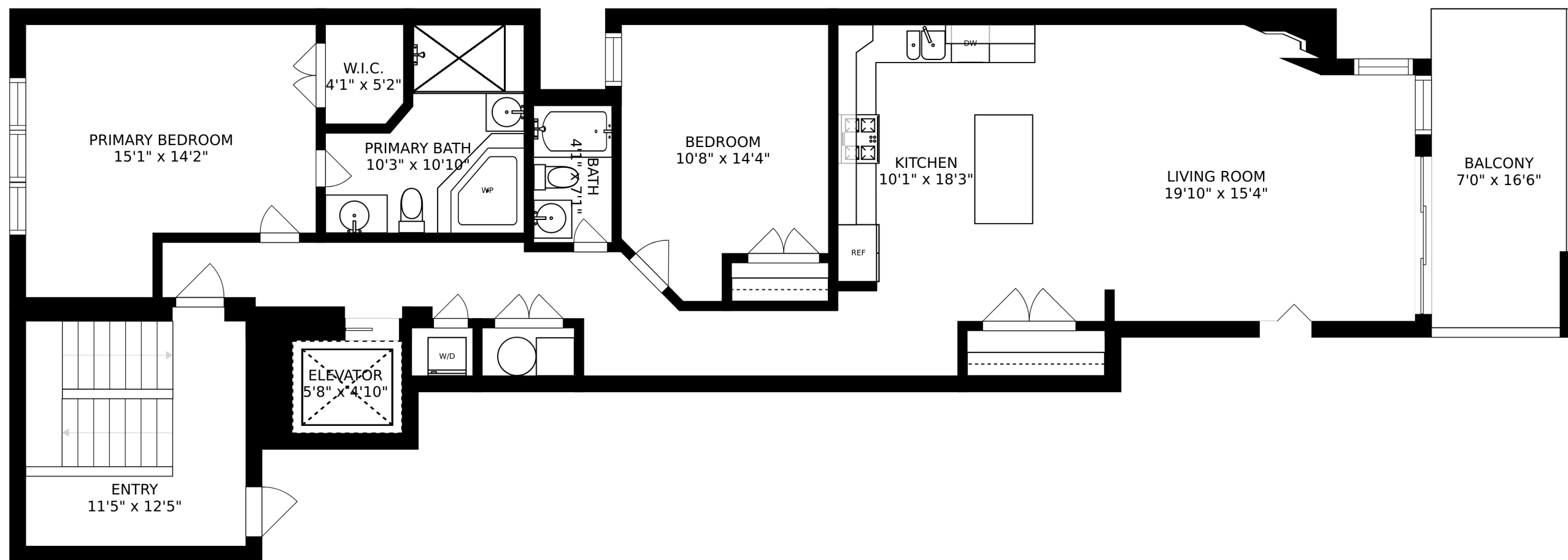
FLOOR 1
