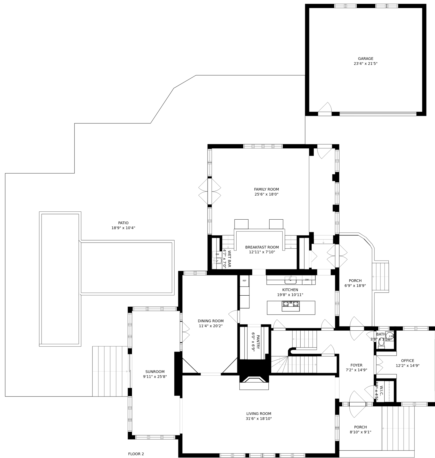
FLOOR 2
