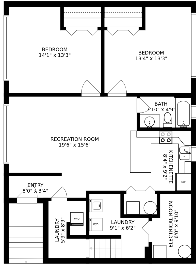
FLOOR 1
