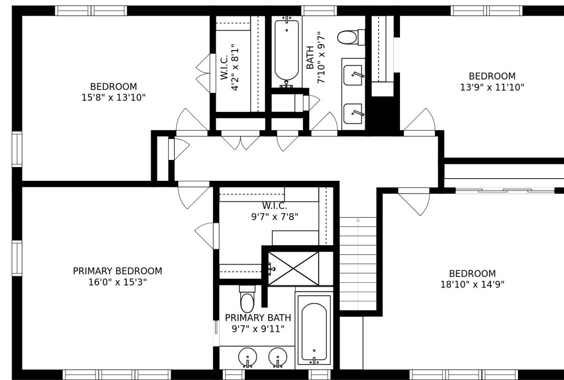
FLOOR 3
