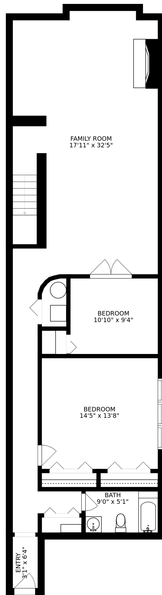
FLOOR 1
