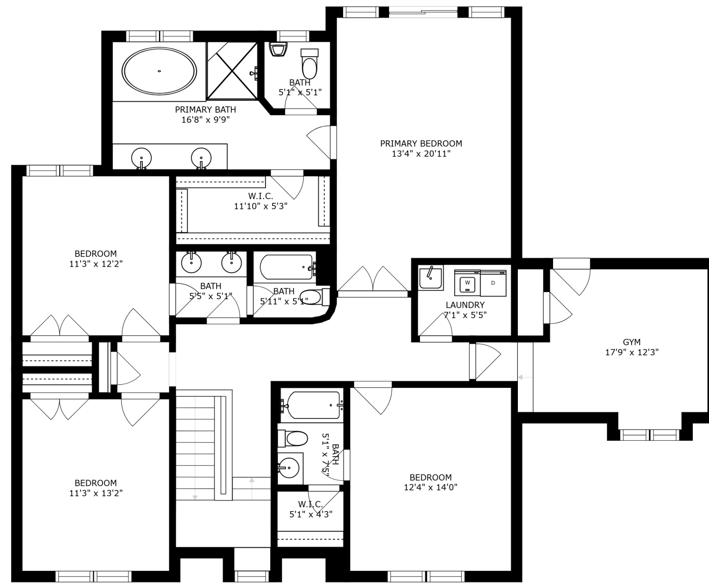
FLOOR 3
