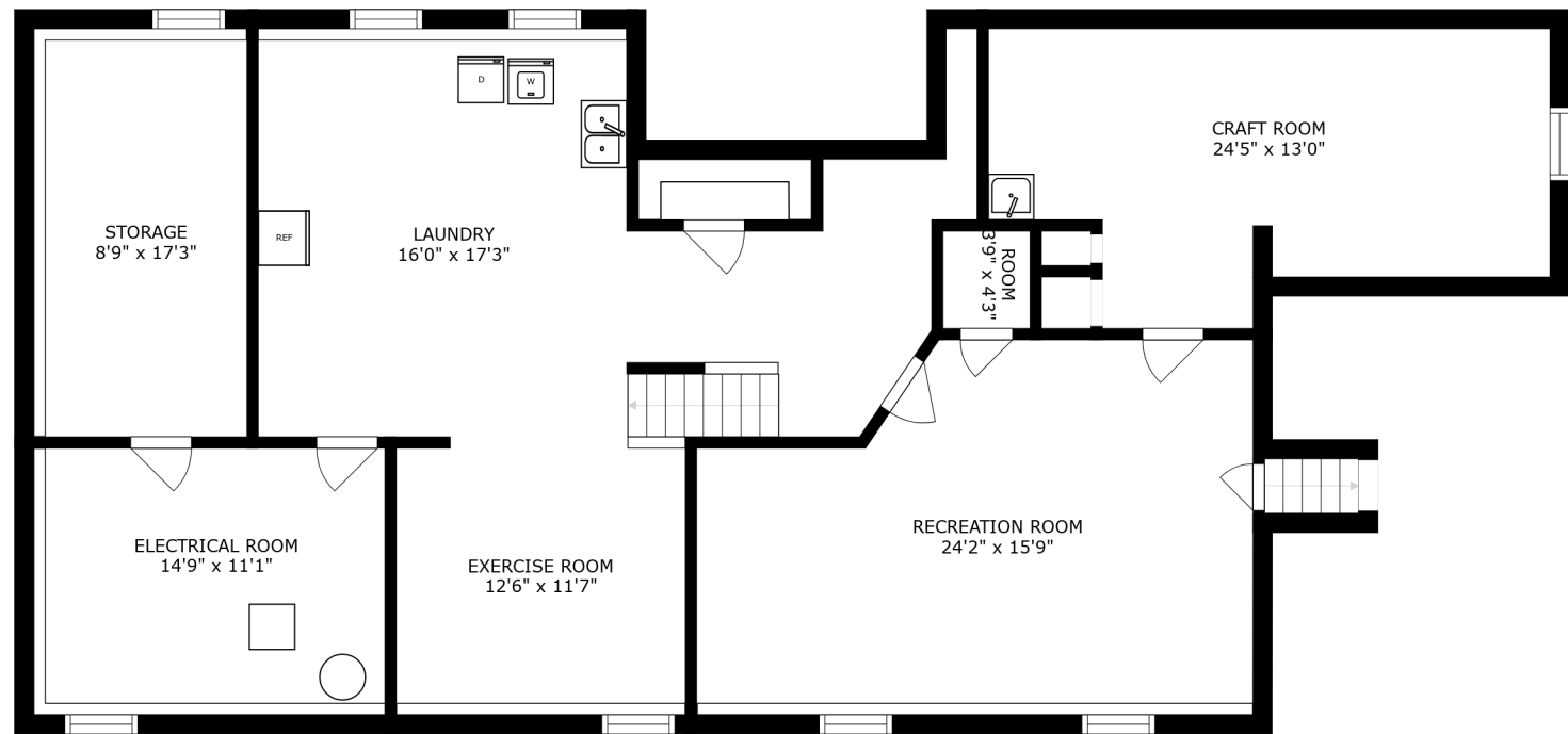
FLOOR 1
