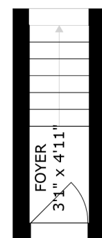
FLOOR 1
