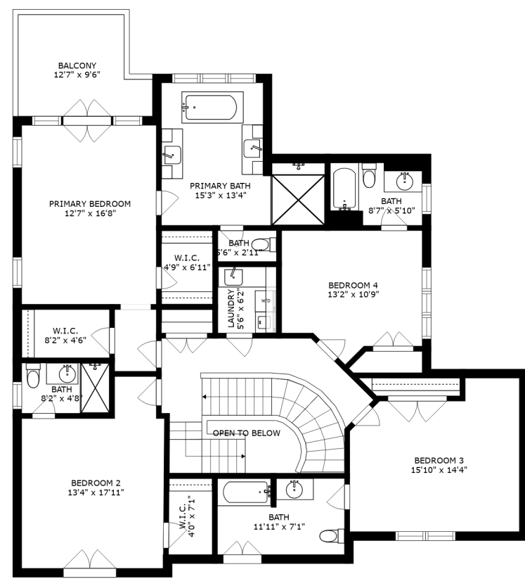
FLOOR 3
