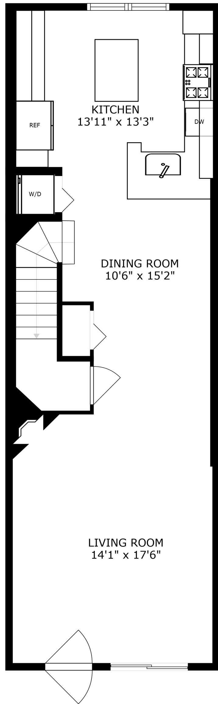
FLOOR 1
