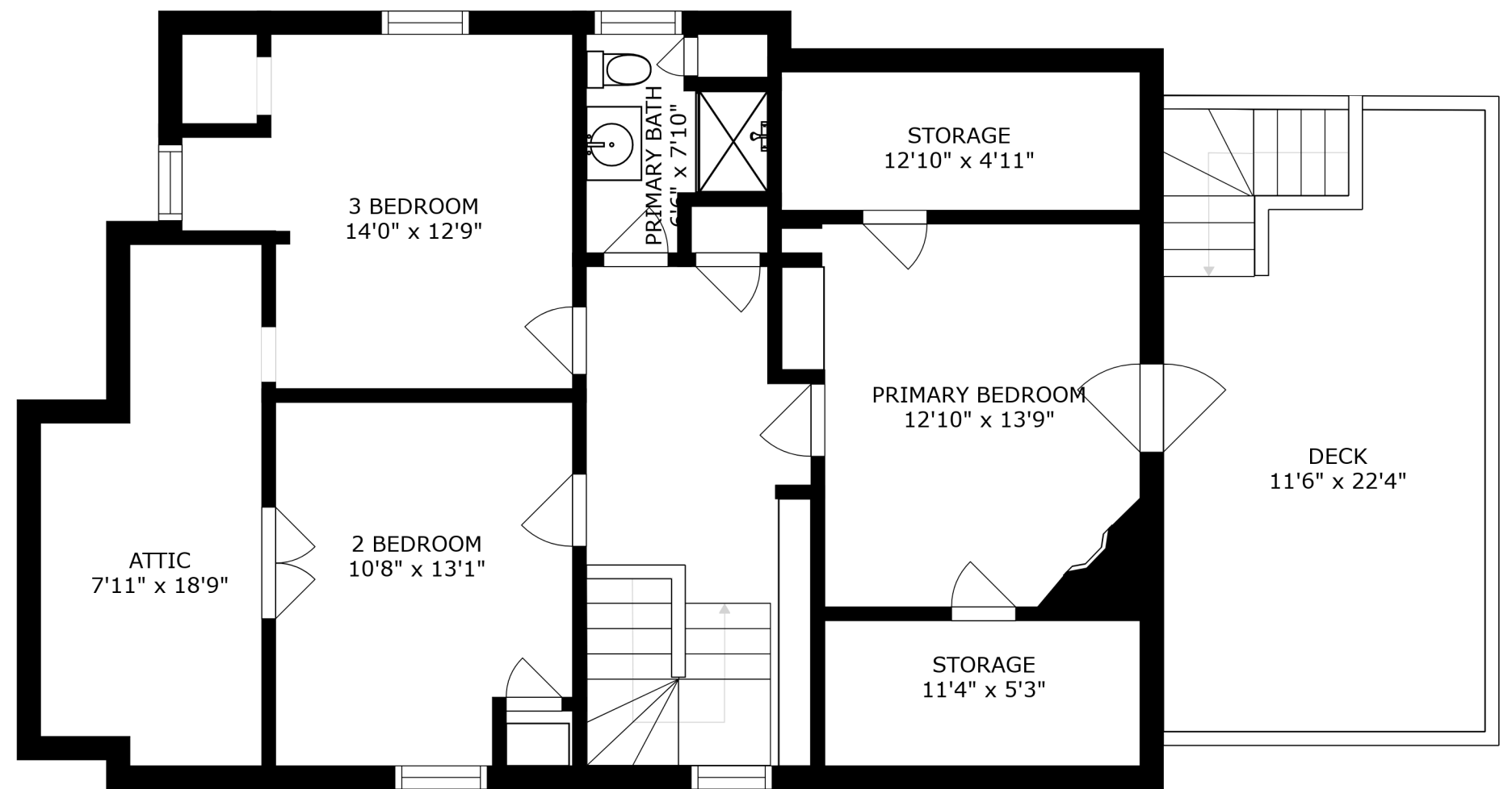
FLOOR 3
