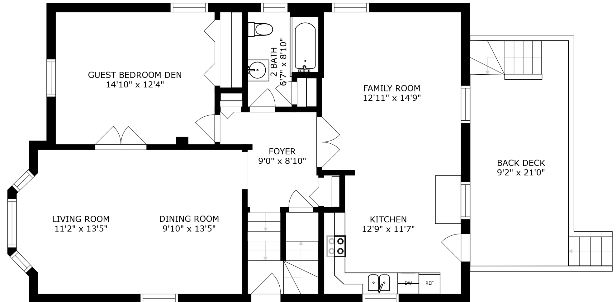
FLOOR 2
