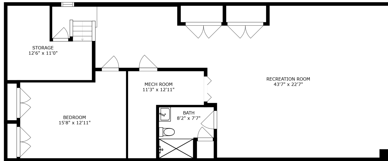
FLOOR 1
