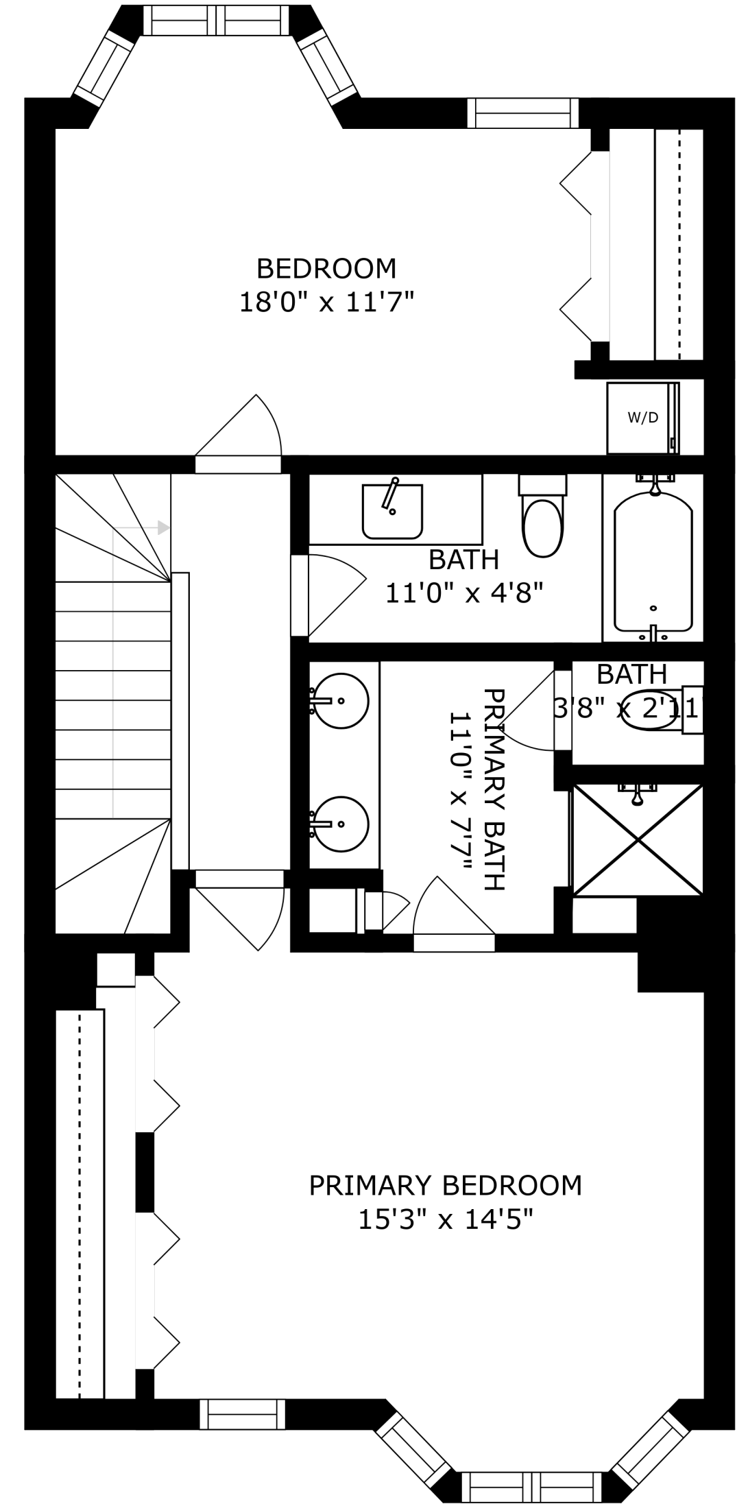
FLOOR 3
