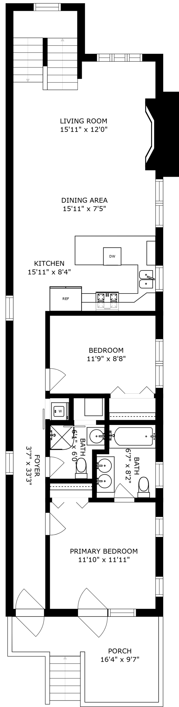
FLOOR 2
