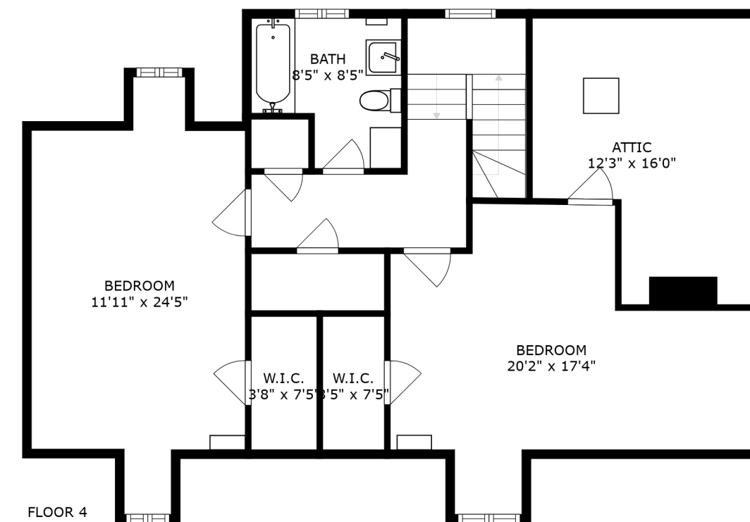
FLOOR 4
