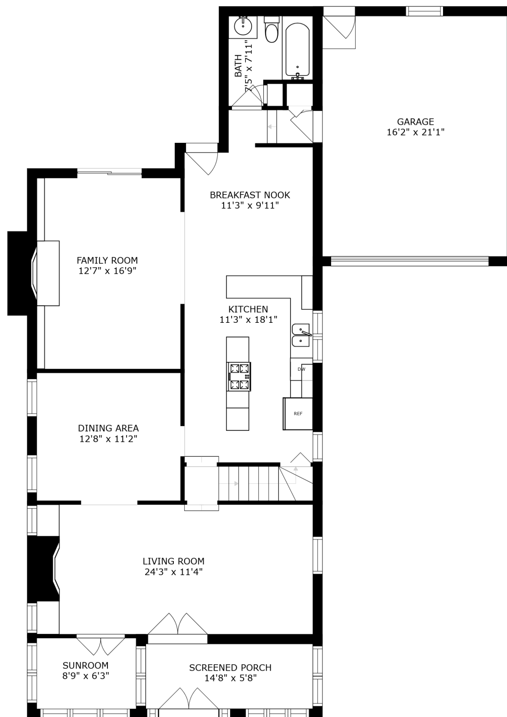
FLOOR 2
