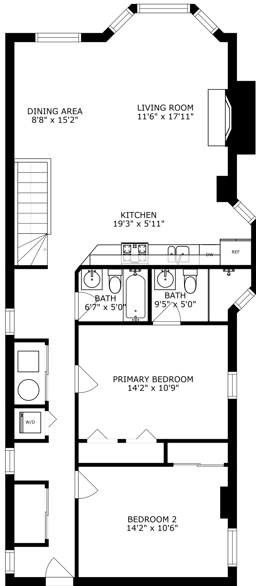
FLOOR 2
