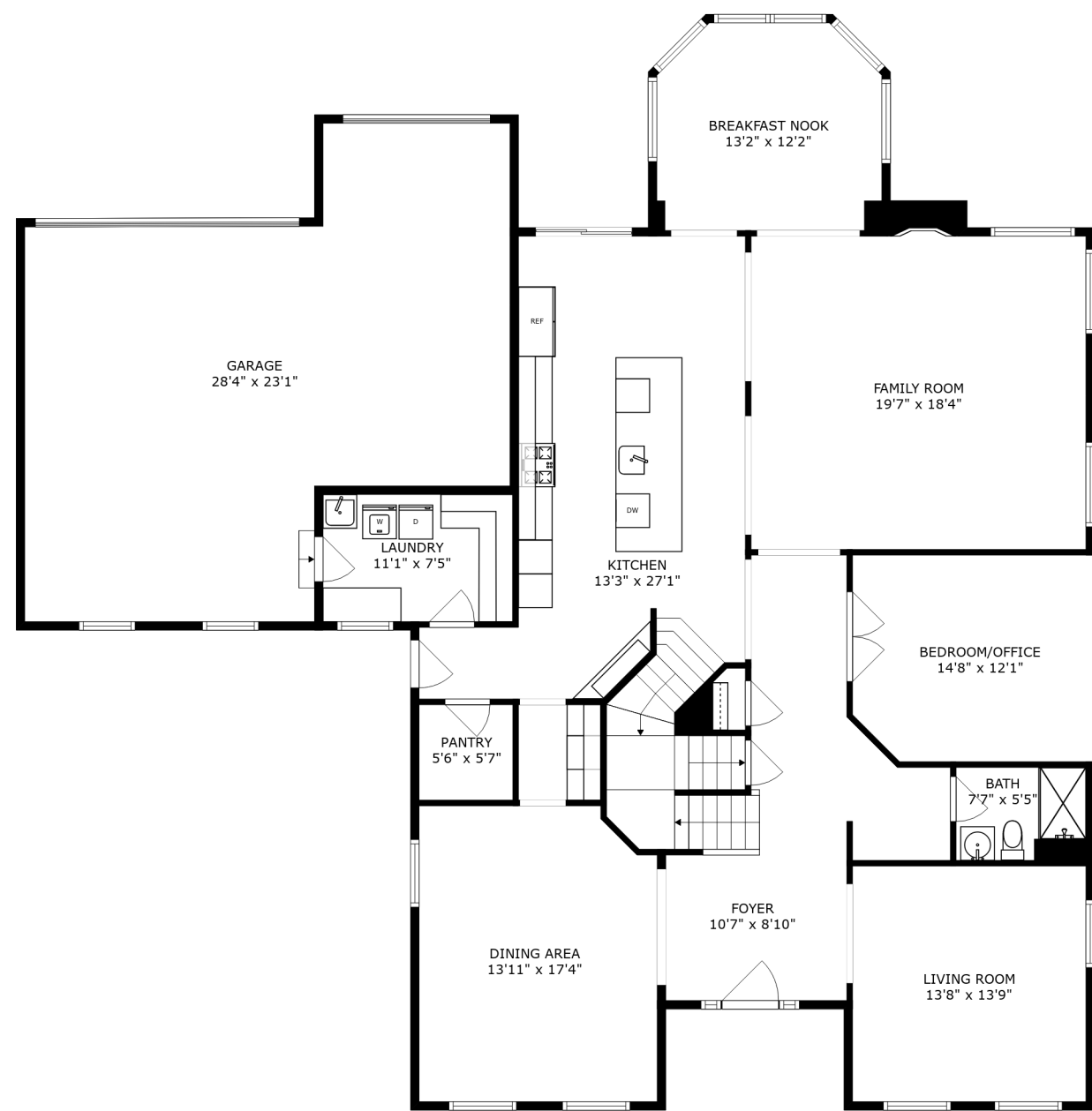
FLOOR 2
