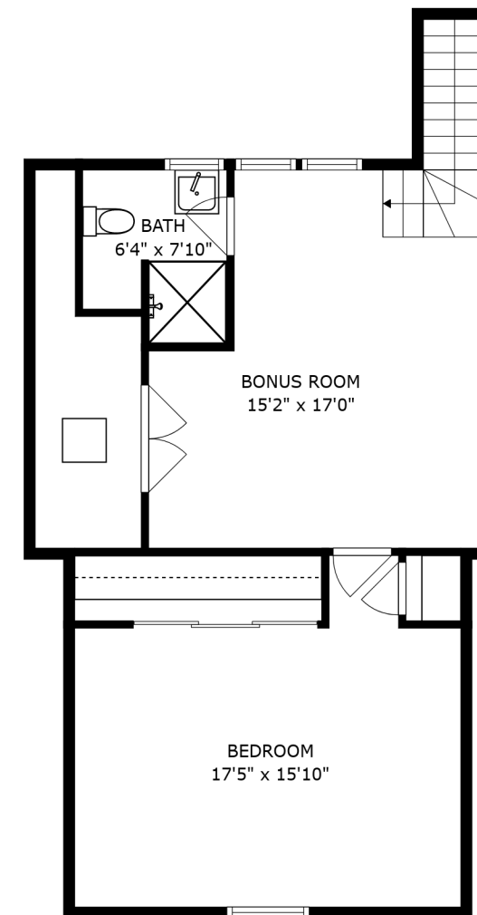
FLOOR 3
