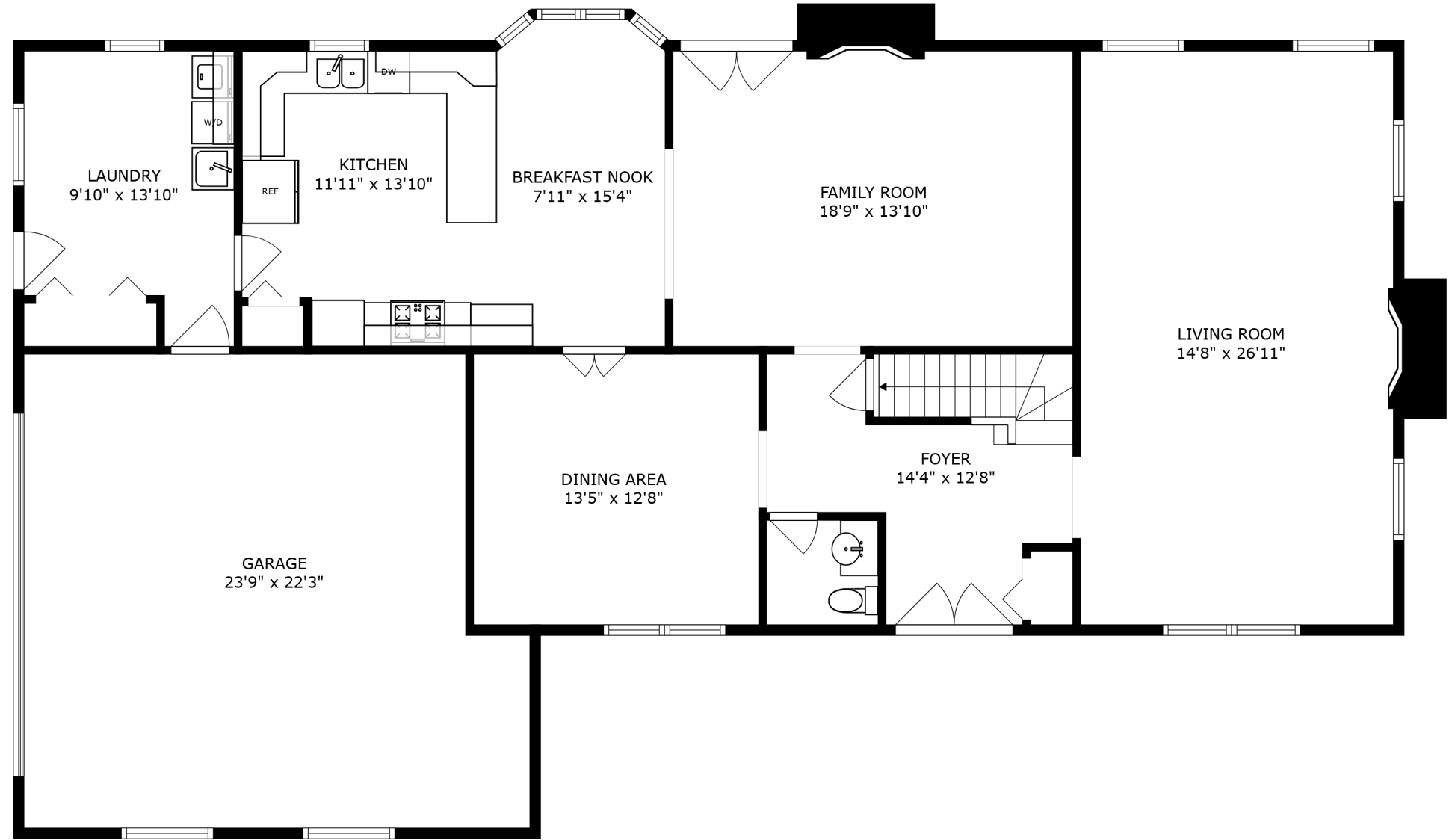
FLOOR 2
