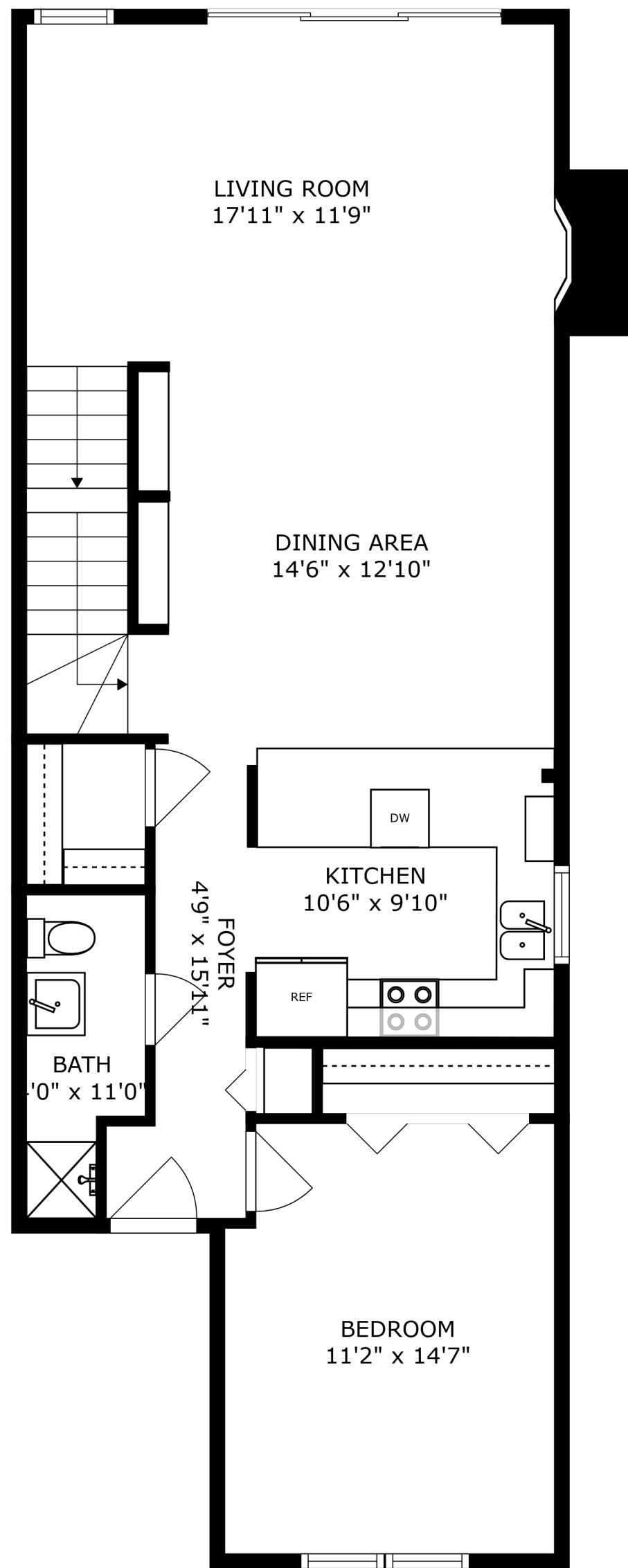
FLOOR 1
