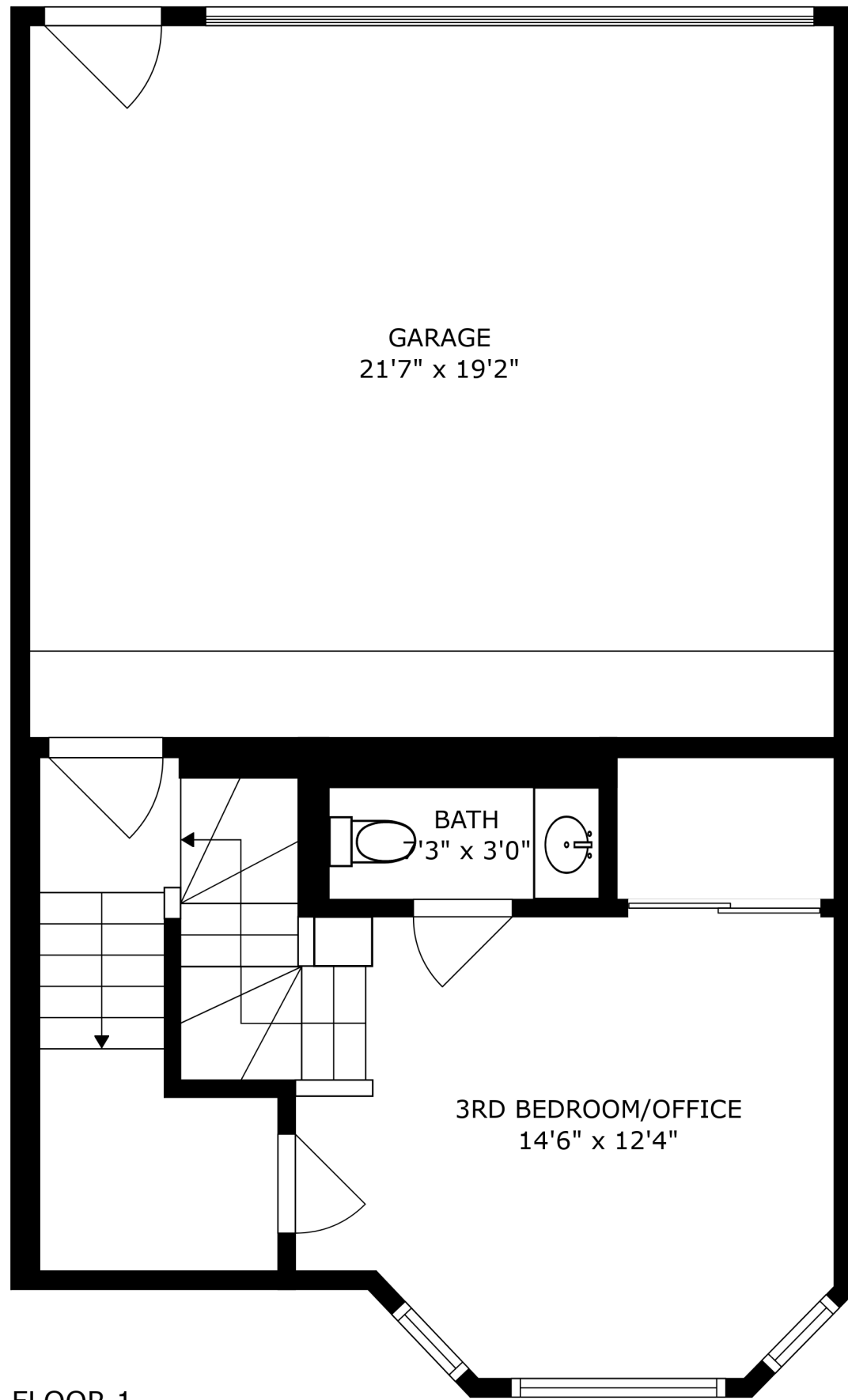
FLOOR 1
