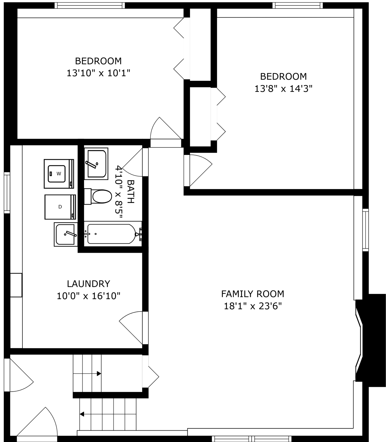
FLOOR 1
