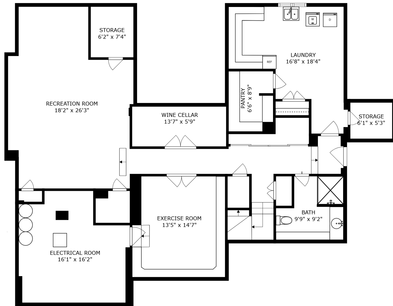
FLOOR 1
