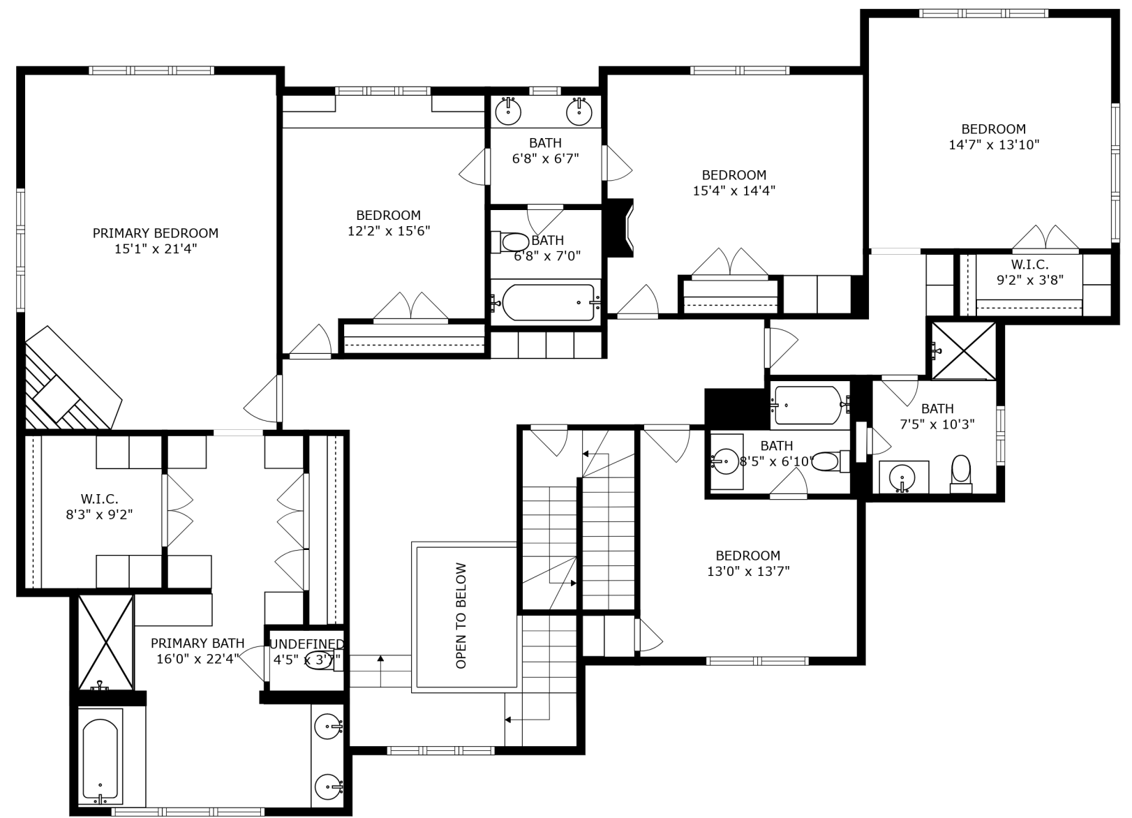
FLOOR 3
