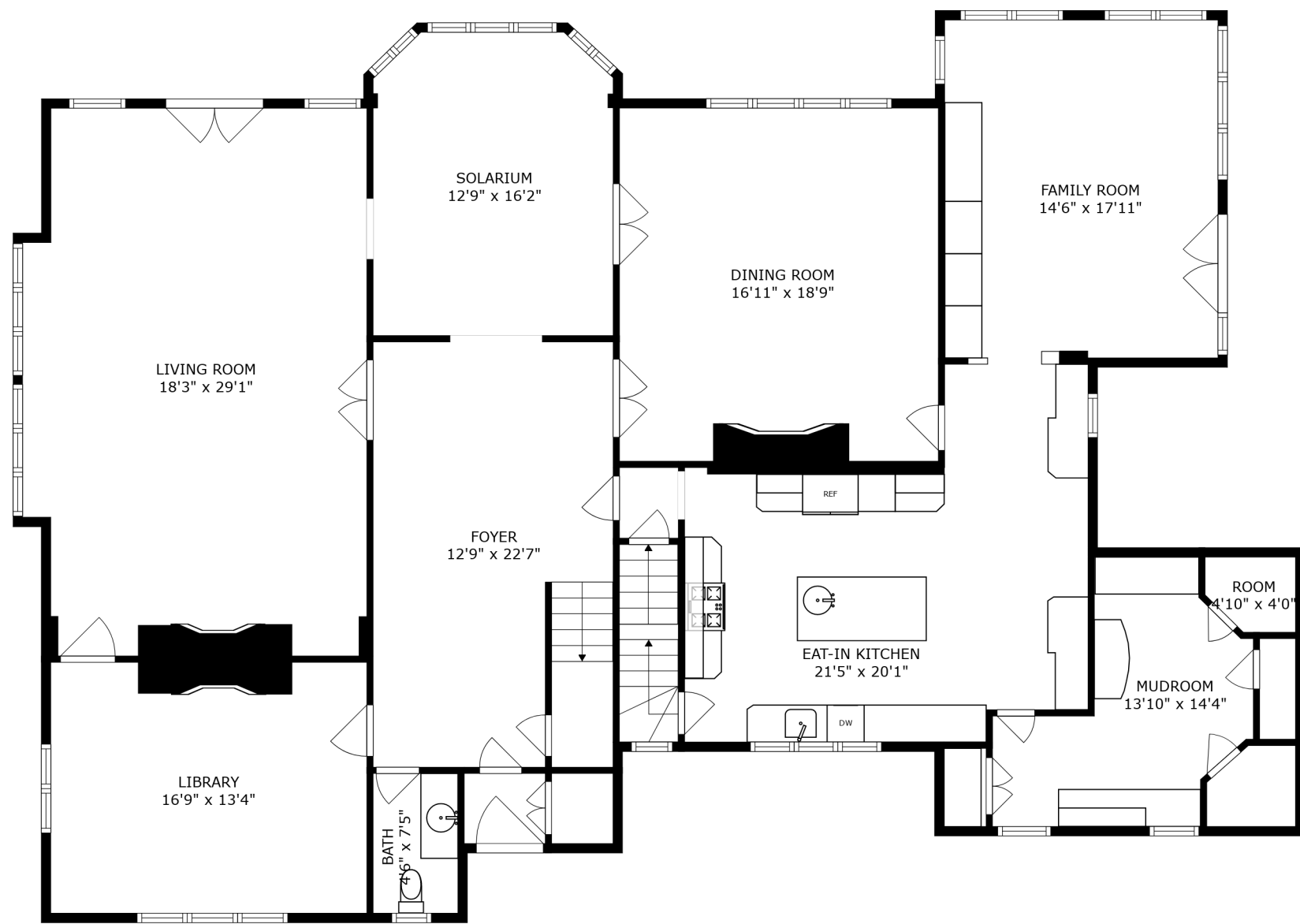
FLOOR 2
