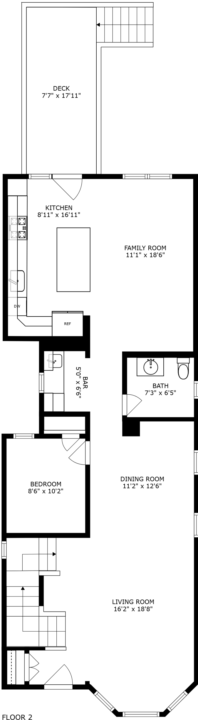
FLOOR 2
