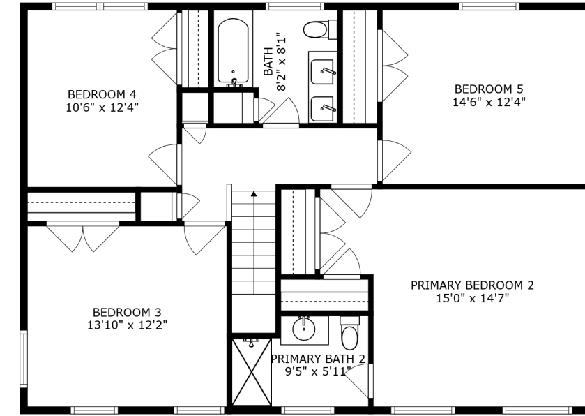
FLOOR 2
