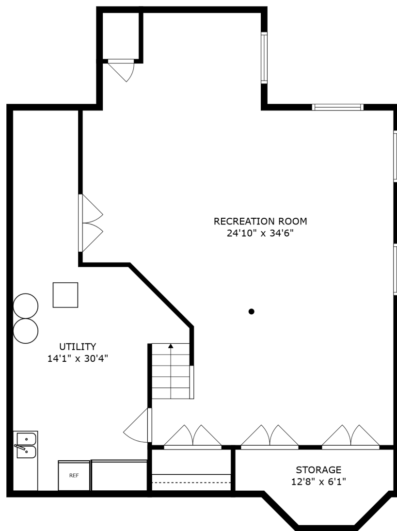
FLOOR 1
