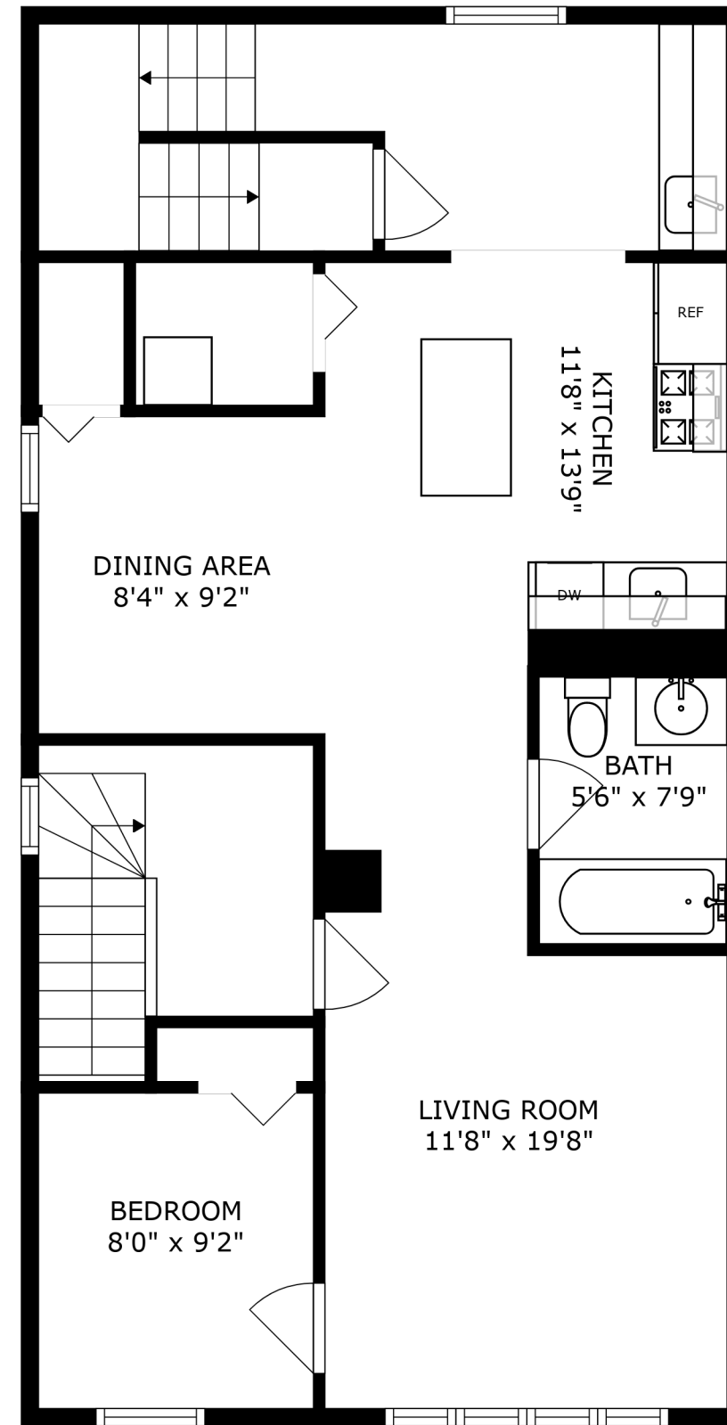
FLOOR 3
