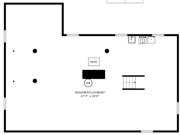
BASEMENT
