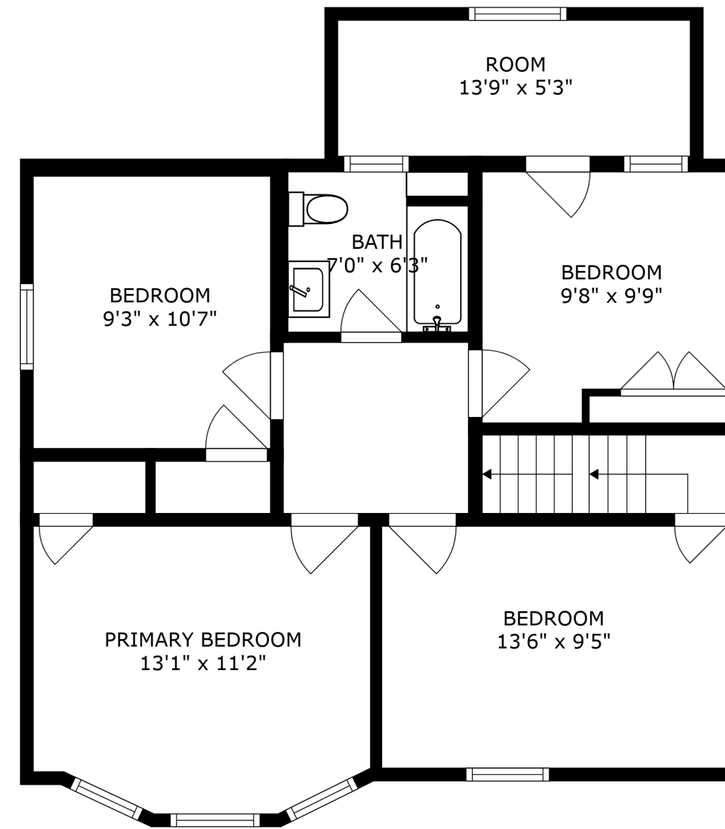
FLOOR 3
