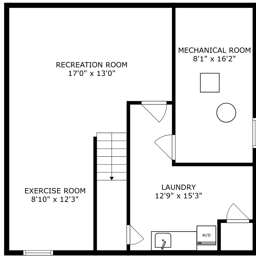
FLOOR 1
