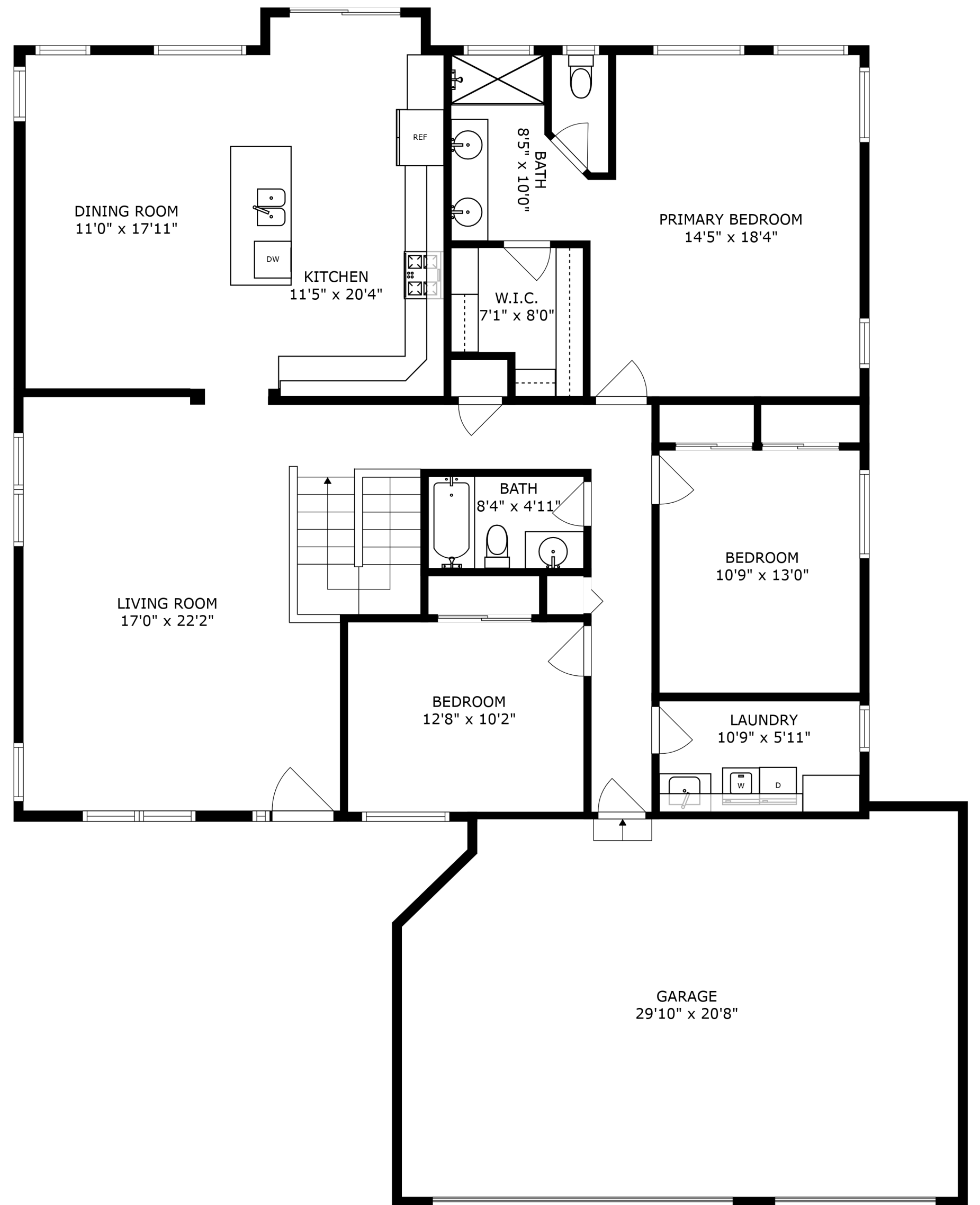
FLOOR 2
