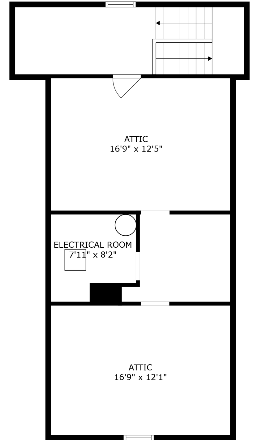
FLOOR 4
