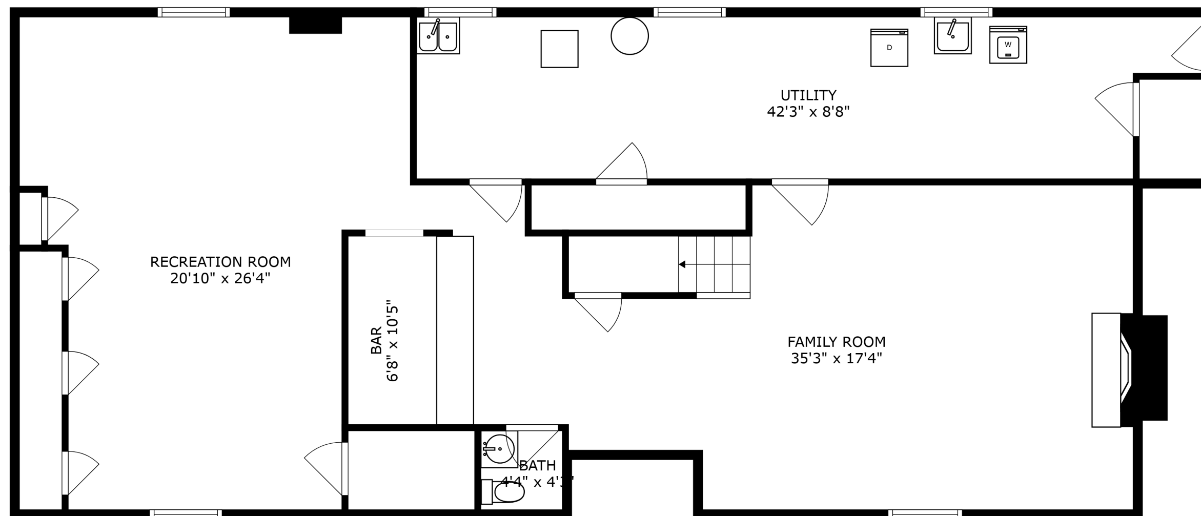
FLOOR 1
