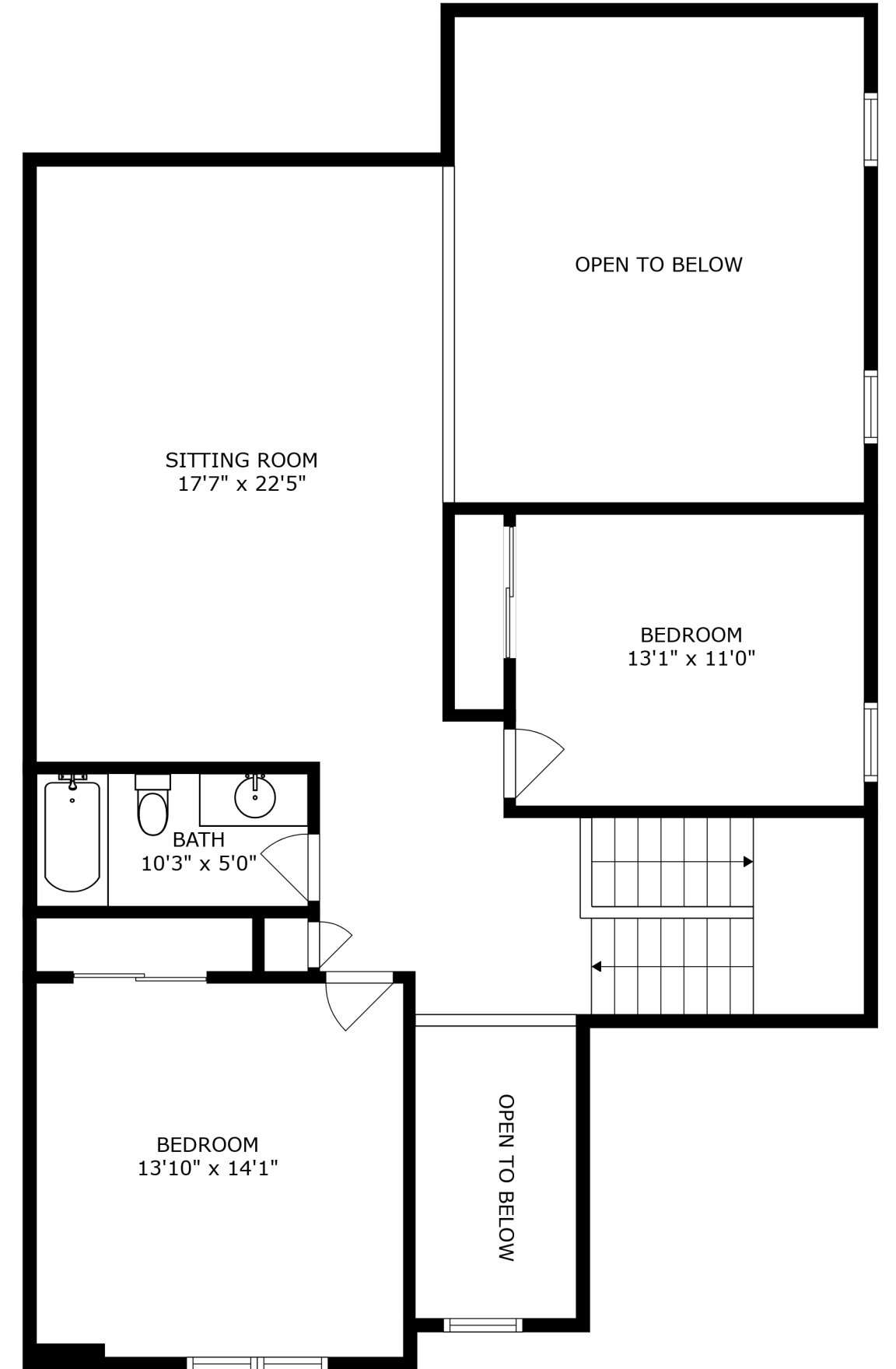
FLOOR 3
