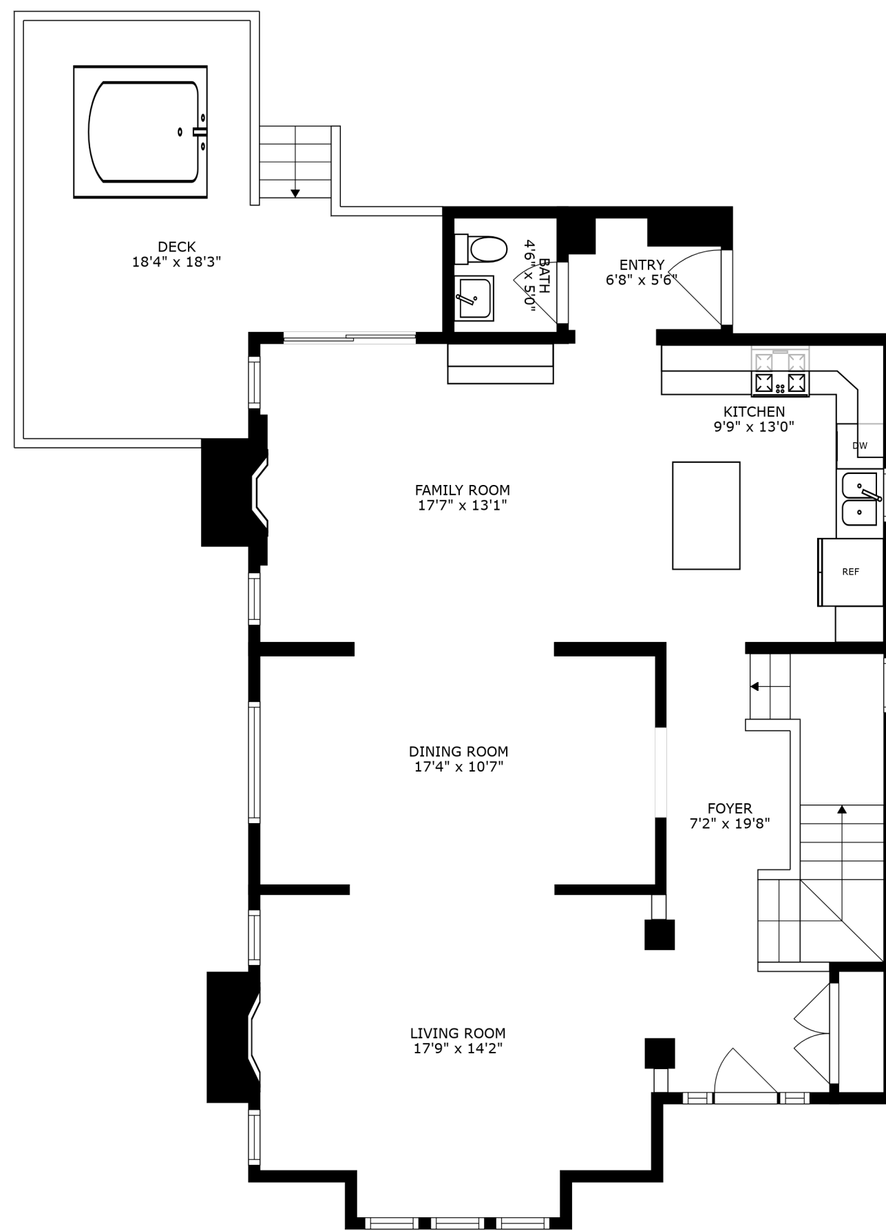
FLOOR 2
