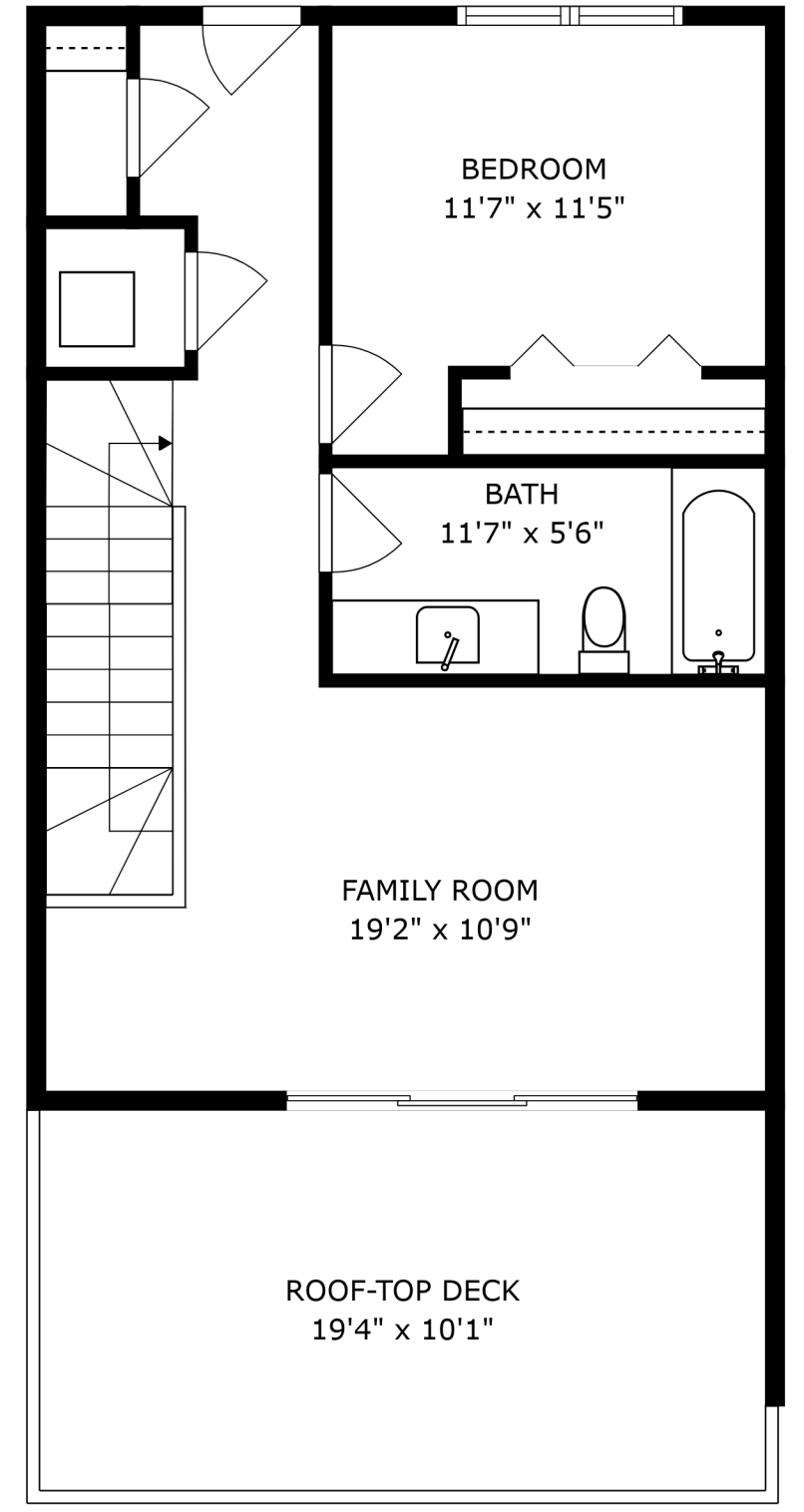
FLOOR 4
