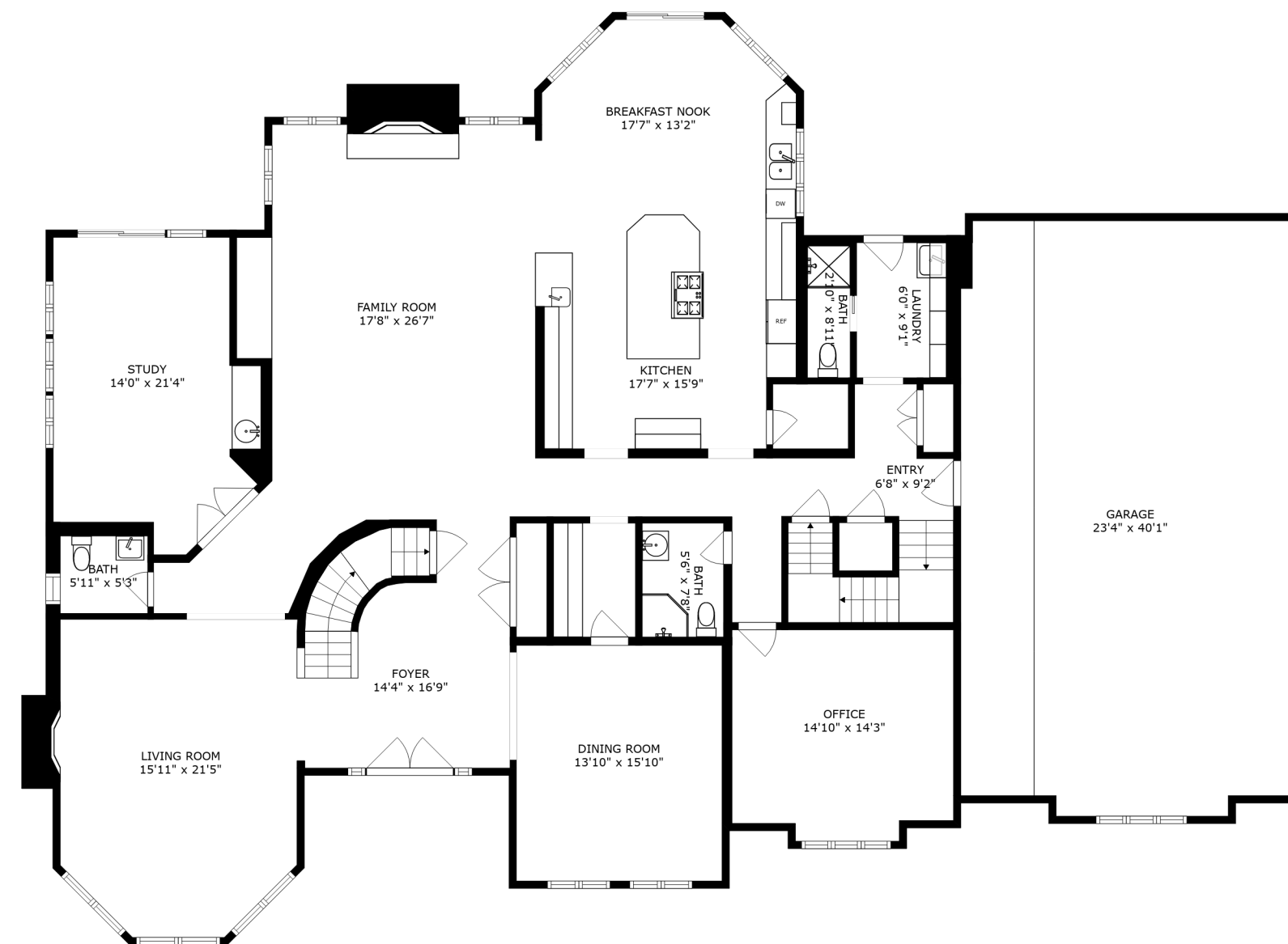
FLOOR 2
