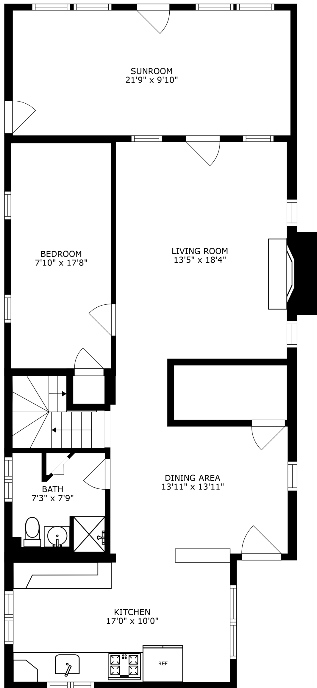
FLOOR 1
