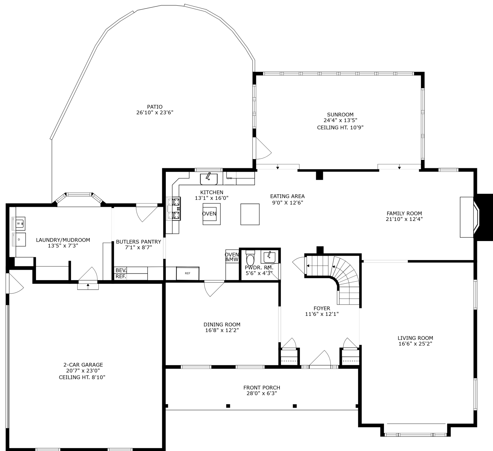
FIRST FLOOR APPROX. INTERIOR SQ. FOOTAGE - 2,043 EXCLUDES GARAGE - 533 CEILING HT. 8'0" UNLESS SPECIFIED
