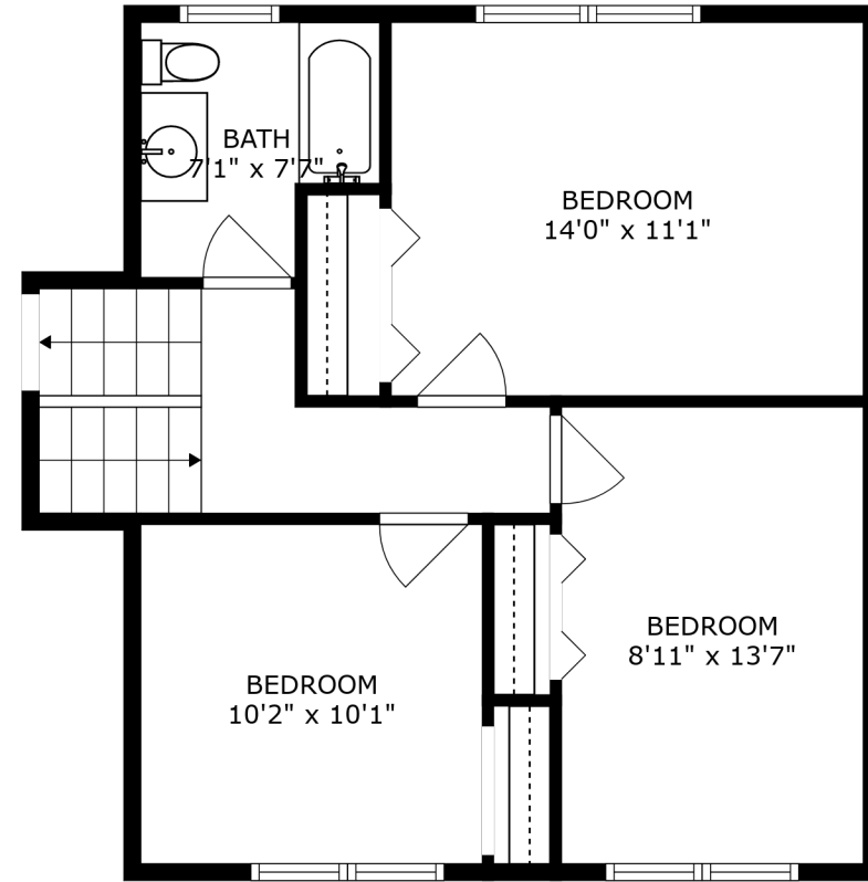
FLOOR 3
