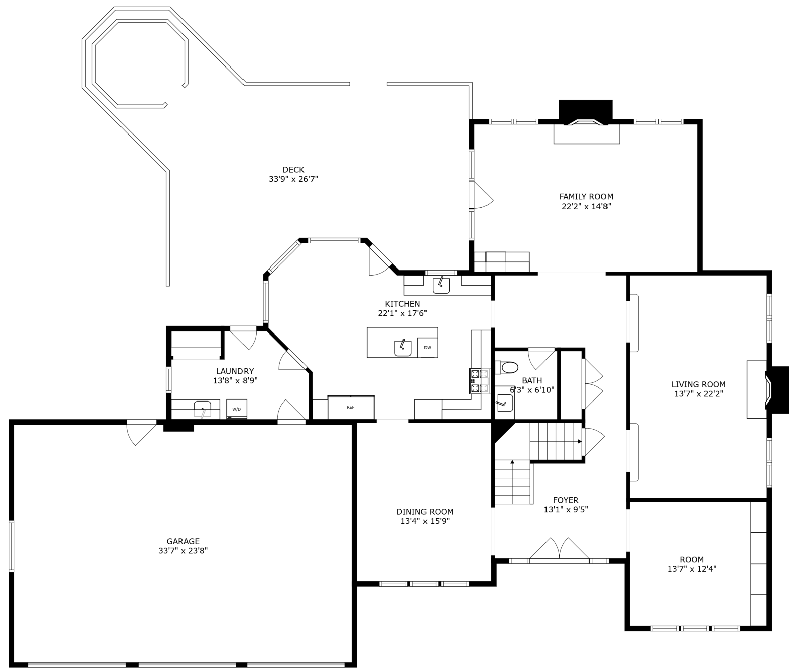
FLOOR 2
