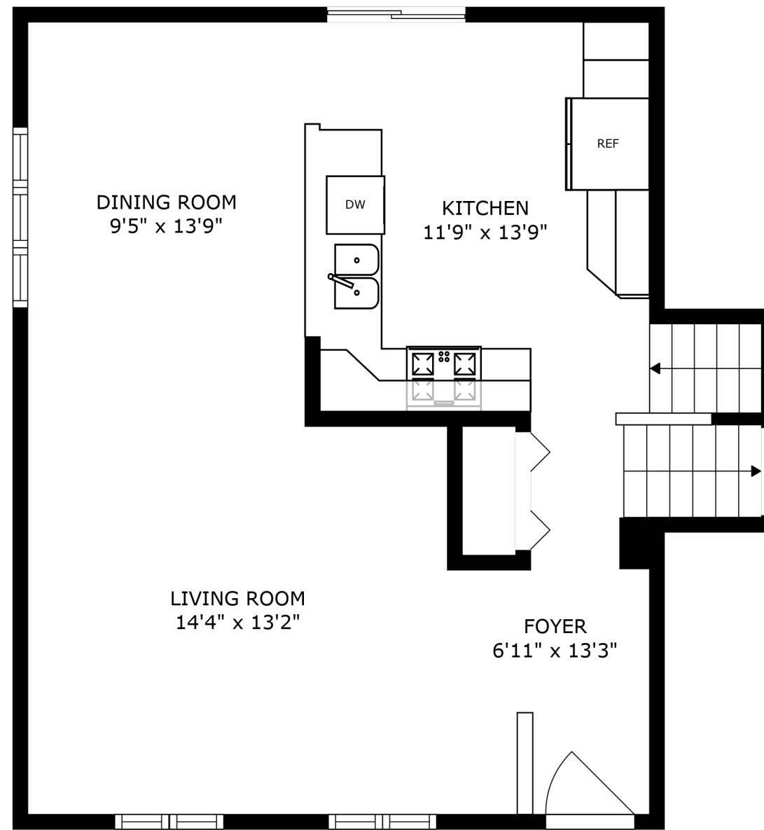
FLOOR 2
