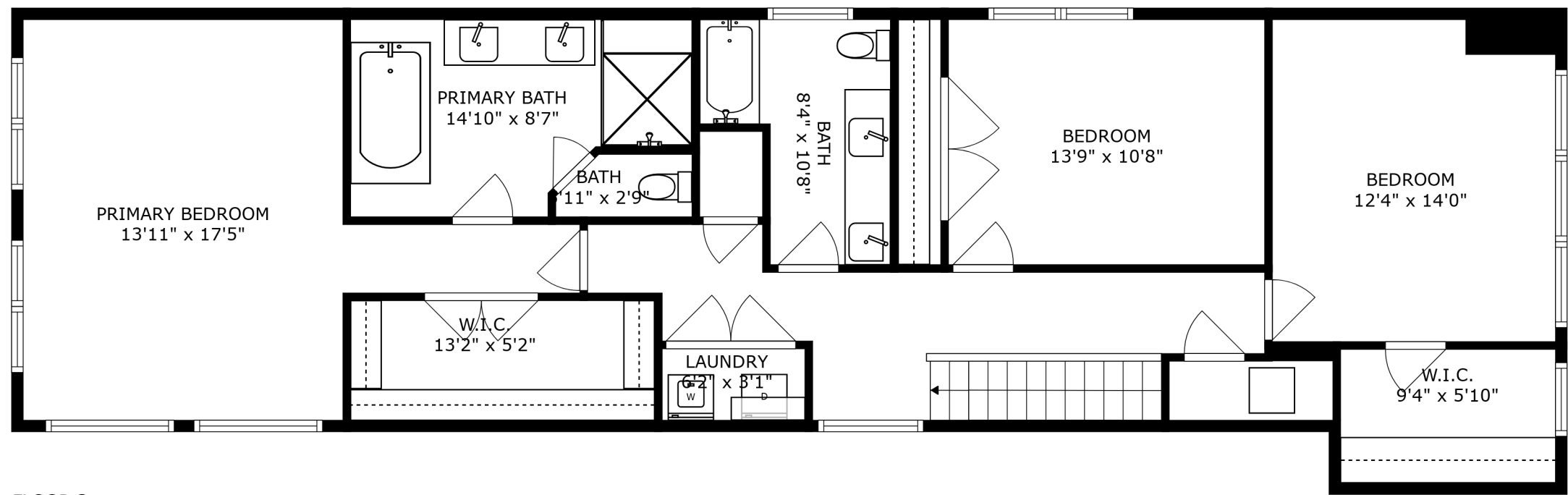
FLOOR 3
