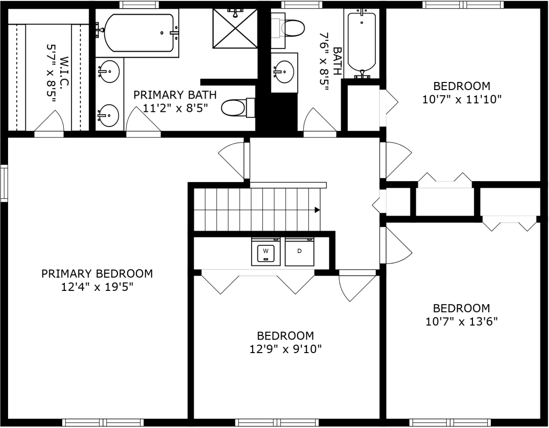
FLOOR 3
