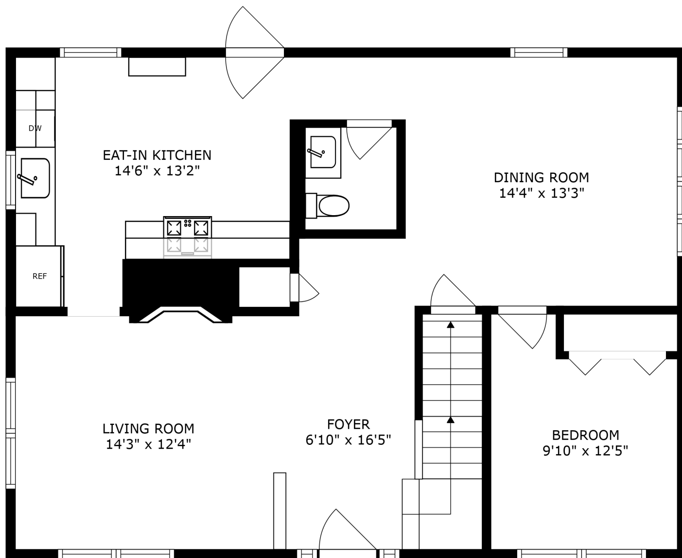
FLOOR 2
