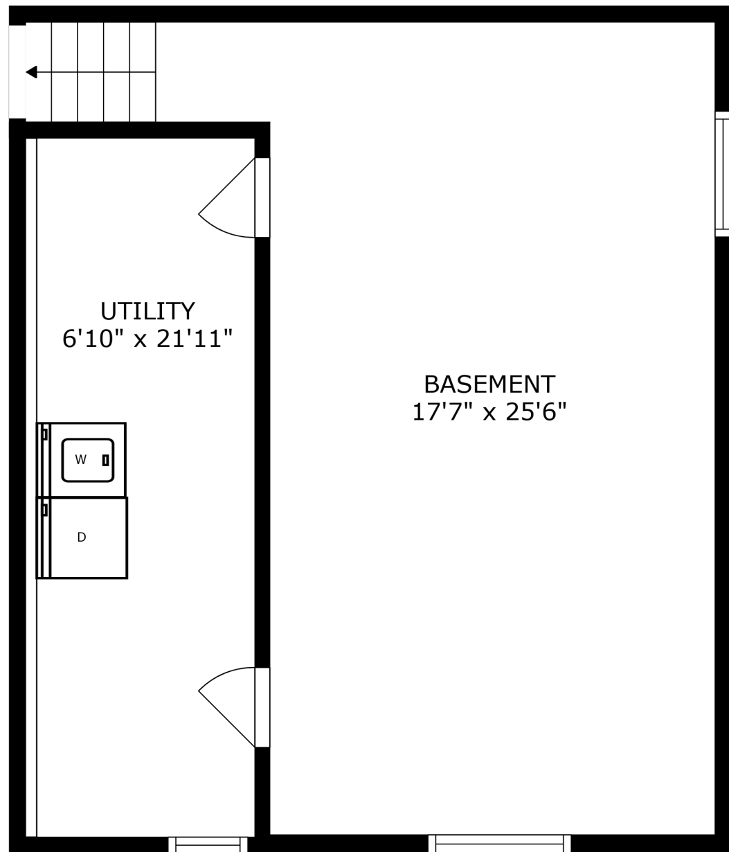
FLOOR 1
